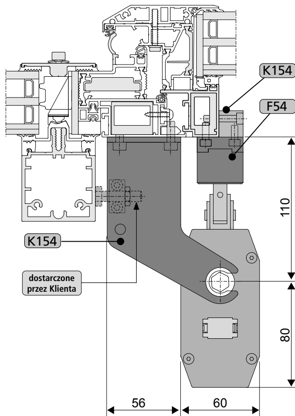
Okno aluminium
